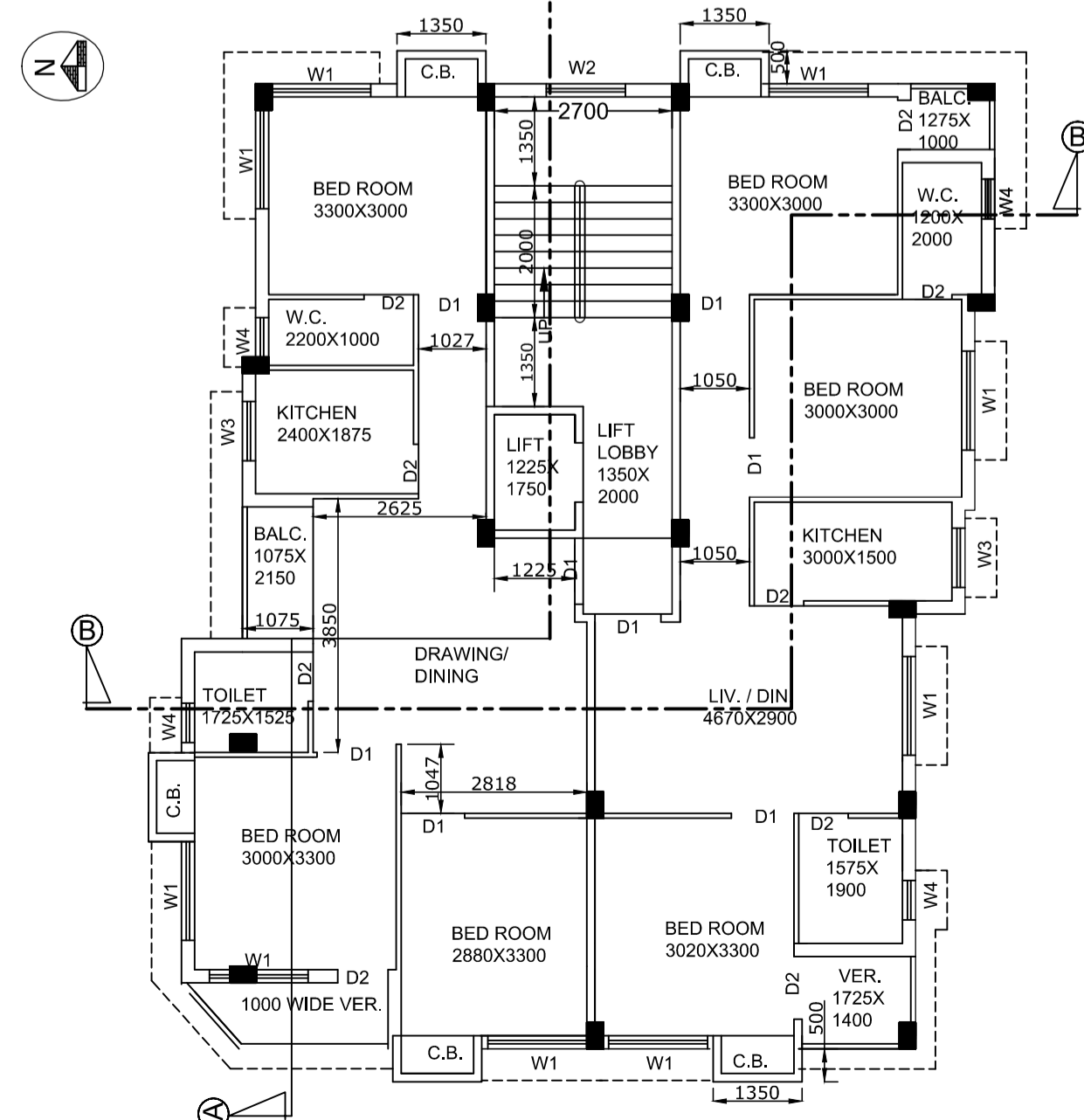
FIRST & THIRD FLOOR PLAN SCALE - 1 : 100
